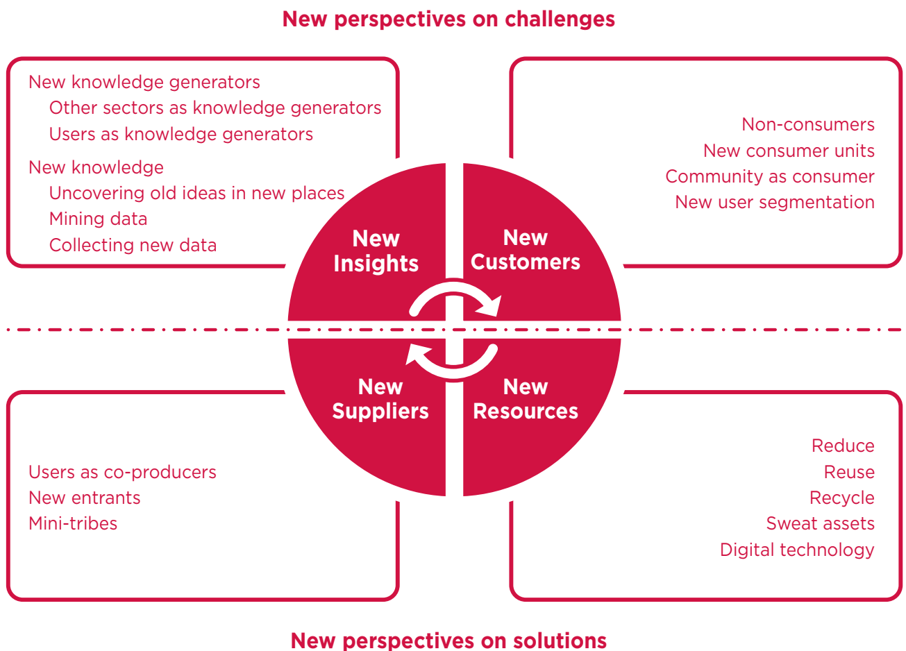
Figure 2. Radical efficiency
